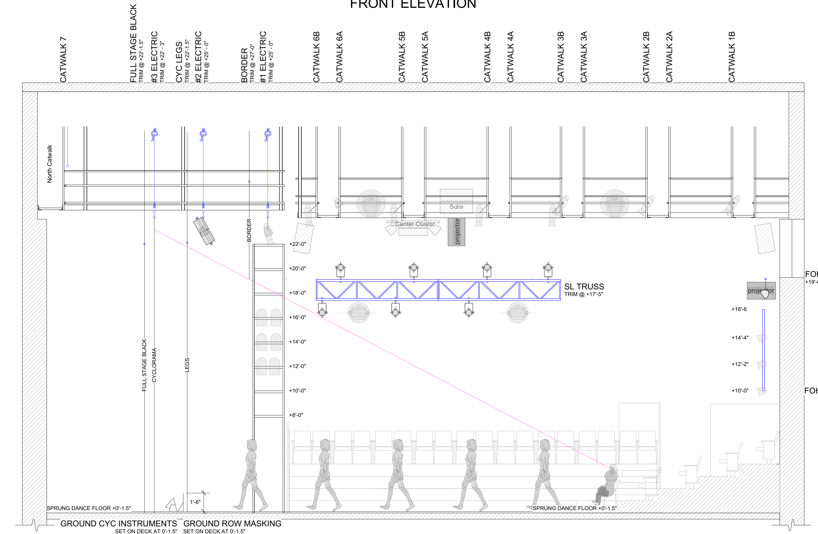
SECTION VIEW FACING STAGE LEFT
