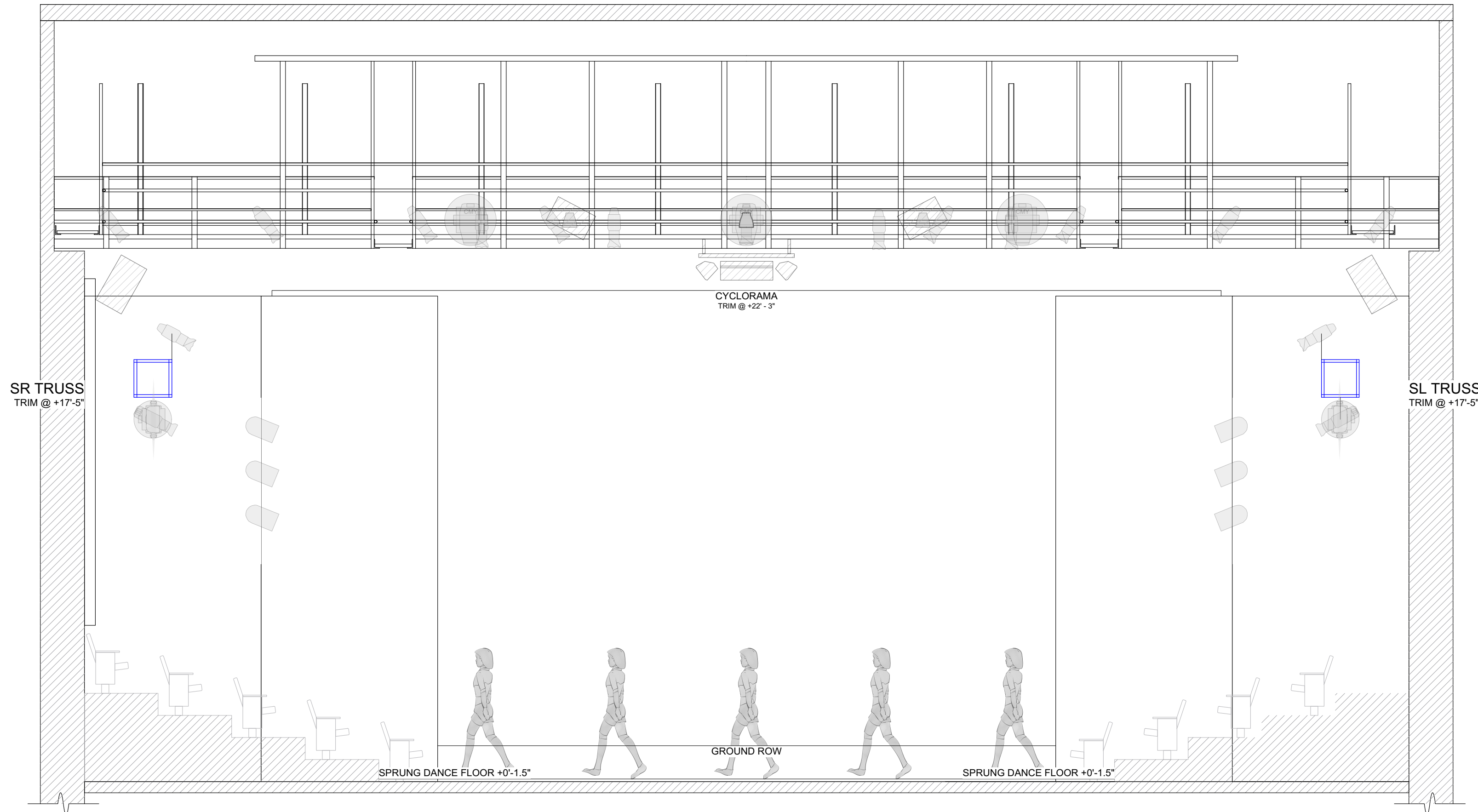
FRONT ELEVATION
